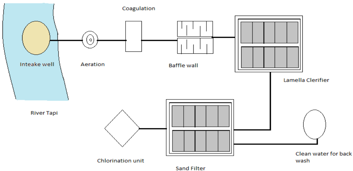
Flowdiagram of Sarthana Water Treatment Plant
