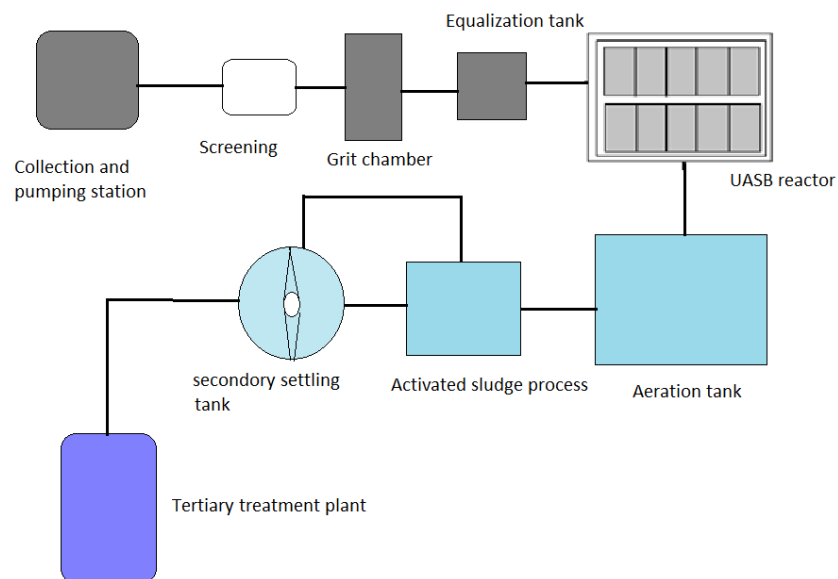
Flow diagram of Bamroli sewage treatment plant.
